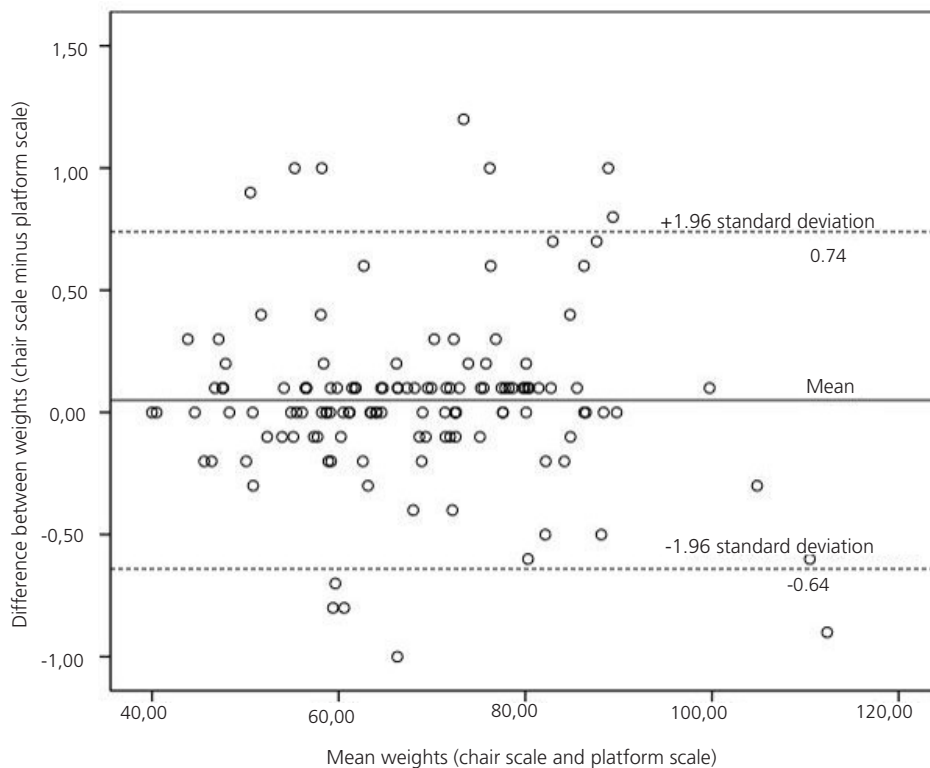
Figure 1 – The Bland-Altman plot of the weight of older adults measured by a digital chair scale and mechanical platform scale.
